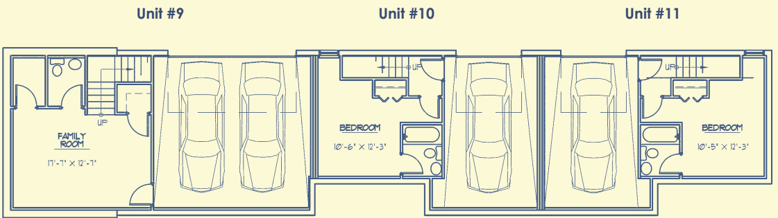
Lower Level
