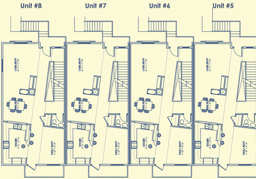
First Level
